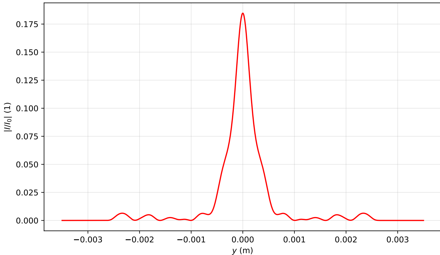
Intensity profile I(x=0, y, z=3.184)/I_0 , Pin=8.0Pcr, artificial time
